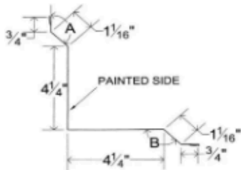
Corner - Inside
