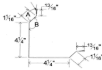
Corner - Outside
