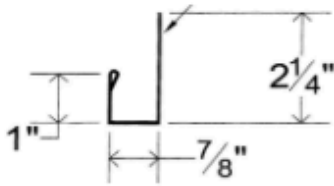
J Flashing
