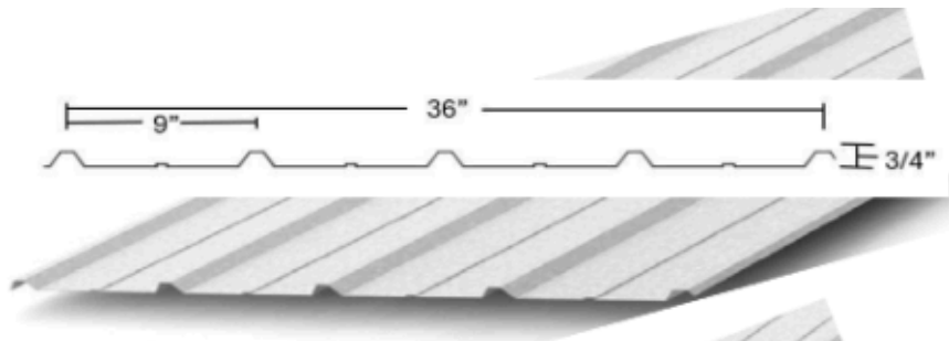
Low Profile
