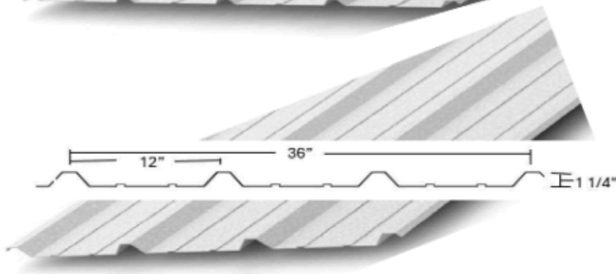
High Profile
