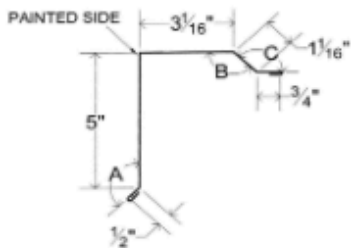
Gable / Rake
