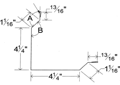
Corner - Outside
