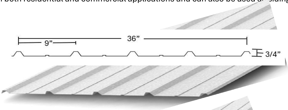
Low Profile
