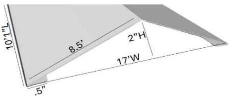
RidgeCap
