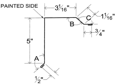
Gable / Rake
