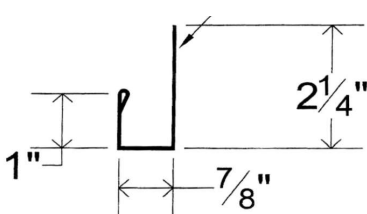
J Flashing
