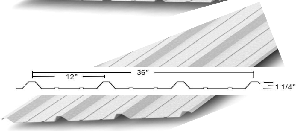
High Profile
