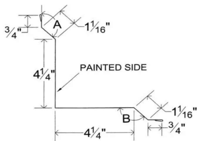
Corner - Inside
