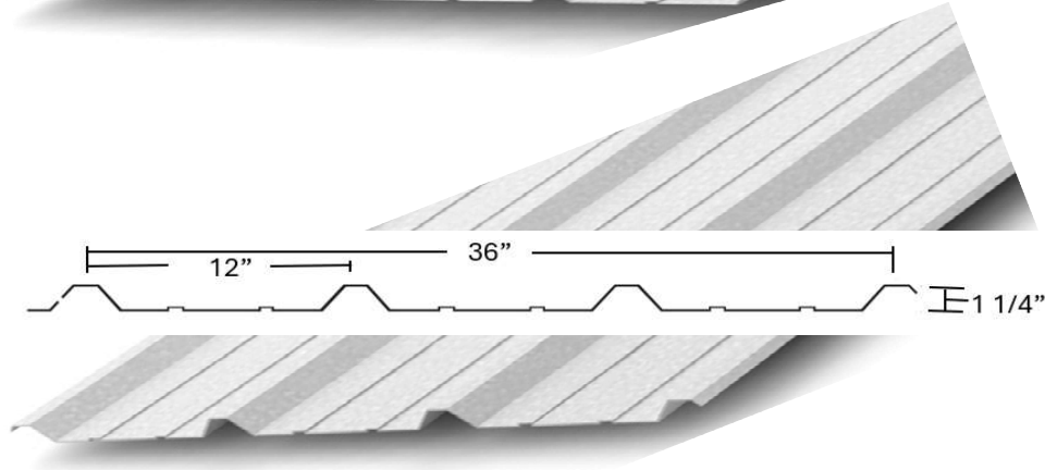
High Profile
