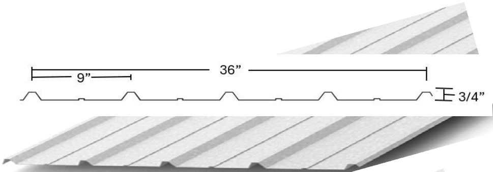
Low Profile
