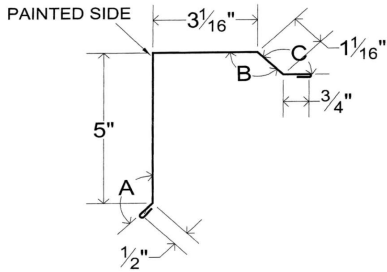
Gable / Rake
