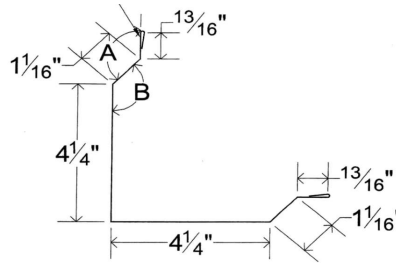
Corner - Outside
