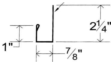
J Flashing
