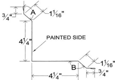
Corner - Inside
